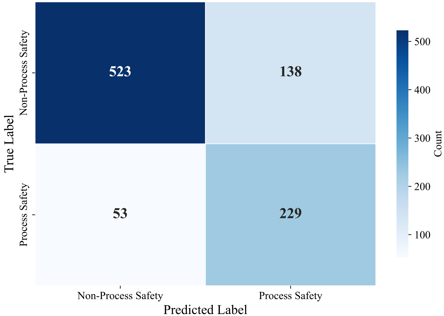
Confusion Matrix — ENGLISH_MANUAL (paraphrase-multilingual-mpnet-base-v2, XGBoost_Optimized)
