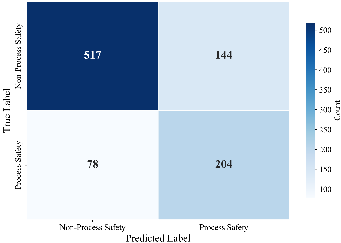
Confusion Matrix — ENGLISH_MANUAL (snowflake-arctic-embed-l-v2.0, SVM)
