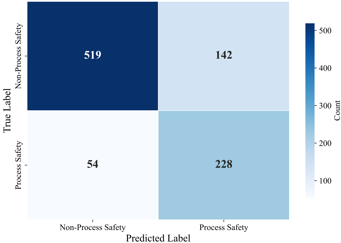
Confusion Matrix — ENGLISH_MANUAL (snowflake-arctic-embed-l-v2.0, Voting_Ensemble)
