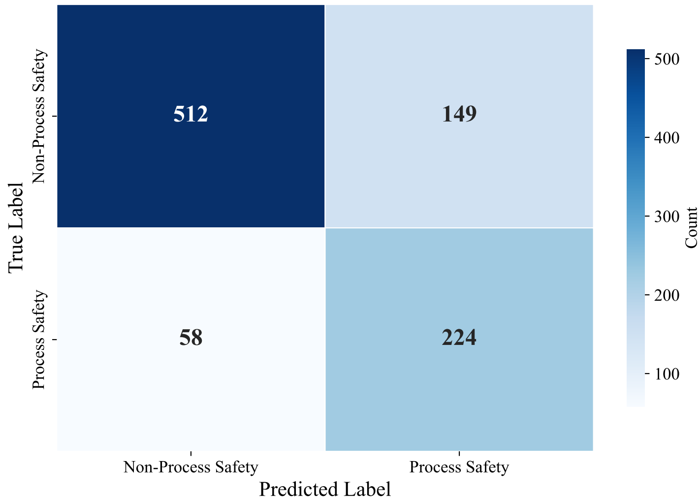
Confusion Matrix — ENGLISH_MANUAL (snowflake-arctic-embed-l-v2.0, XGBoost_Optimized)
