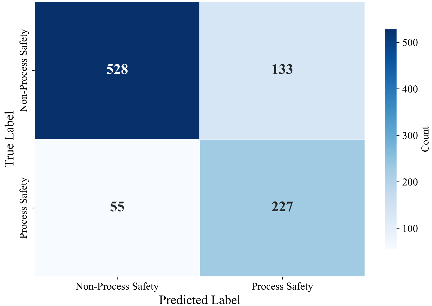
Confusion Matrix — ENGLISH_MANUAL (upskyy/bge-m3-korean, LightGBM_Optimized)
