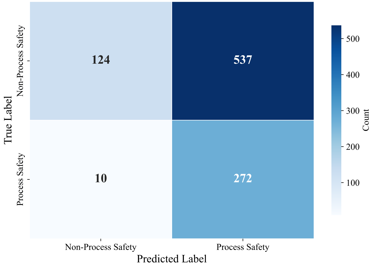
Confusion Matrix — ENGLISH_MANUAL (upskyy/bge-m3-korean, Random_Forest_Optimized)
