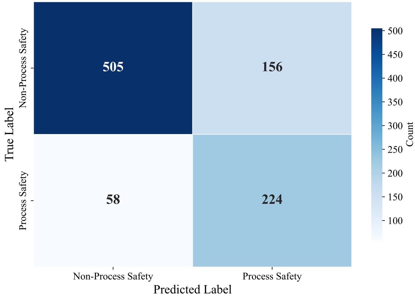
Confusion Matrix — ENGLISH_MANUAL (xlm-roberta-base, Voting_Ensemble)
