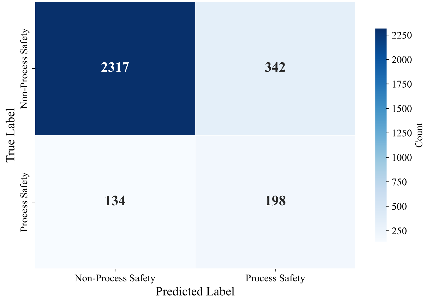
Confusion Matrix — GERMAN_MANUAL (bert-base-multilingual-uncased, LightGBM)
