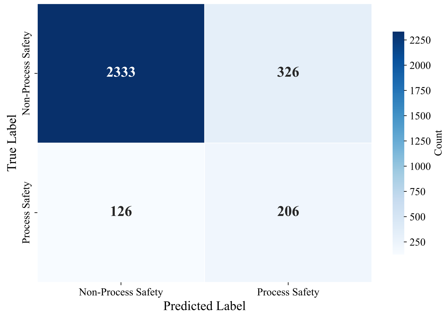
Confusion Matrix — GERMAN_MANUAL (efederici/e5-base-multilingual-4096, XGBoost_Optimized)
