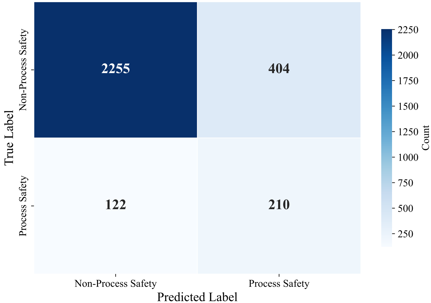
Confusion Matrix — GERMAN_MANUAL (intfloat/multilingual-e5-large-instruct, SVM)
