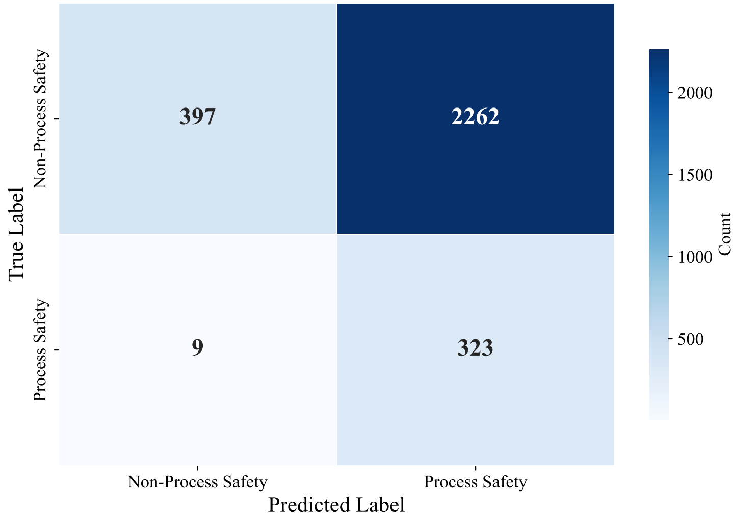
Confusion Matrix — GERMAN_MANUAL (paraphrase-multilingual-MiniLM-L12-v2, Random_Forest_Optimized)
