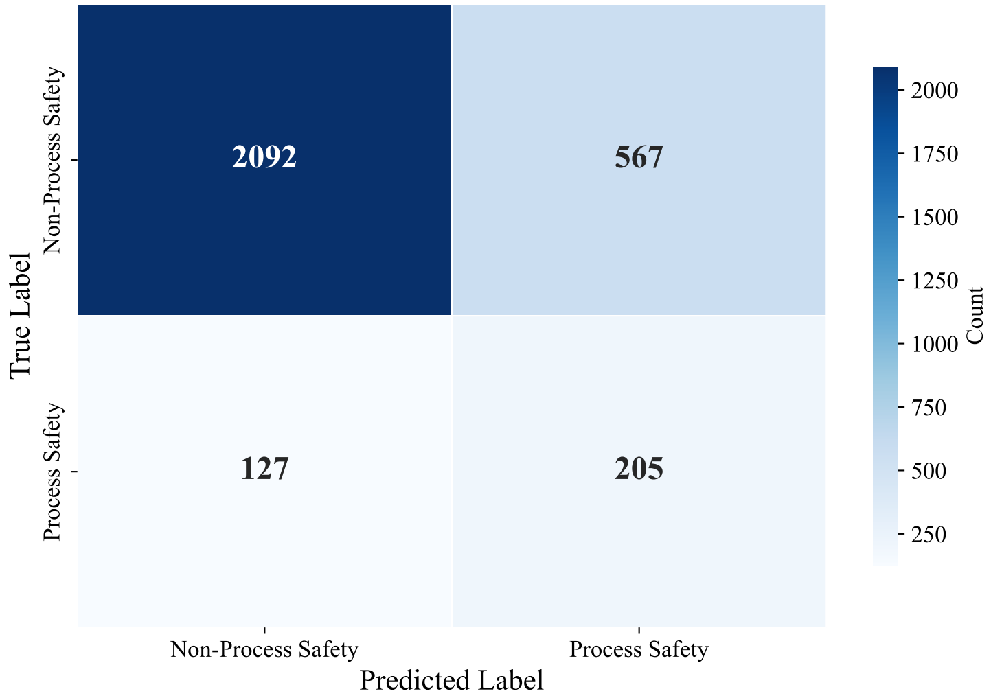
Confusion Matrix — GERMAN_MANUAL (paraphrase-multilingual-MiniLM-L12-v2, SVM)
