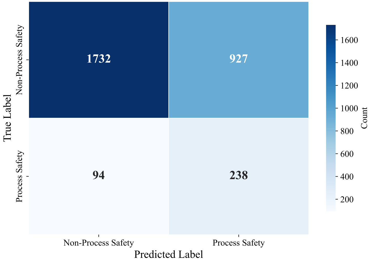
Confusion Matrix — GERMAN_MANUAL (paraphrase-multilingual-mpnet-base-v2, Random_Forest)
