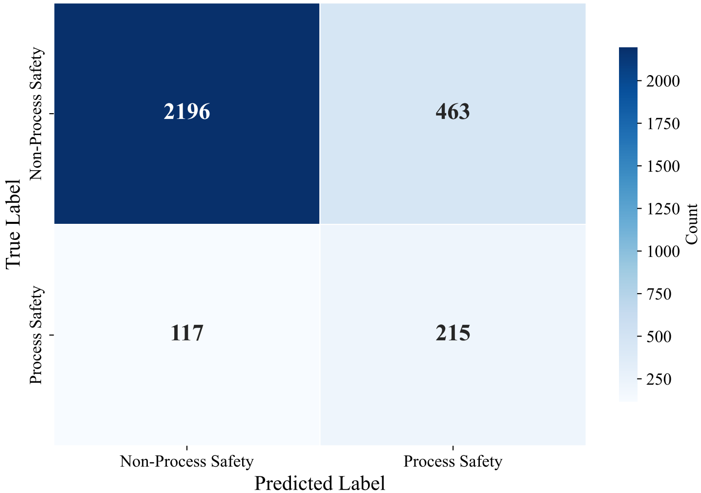
Confusion Matrix — GERMAN_MANUAL (paraphrase-multilingual-mpnet-base-v2, SVM)
