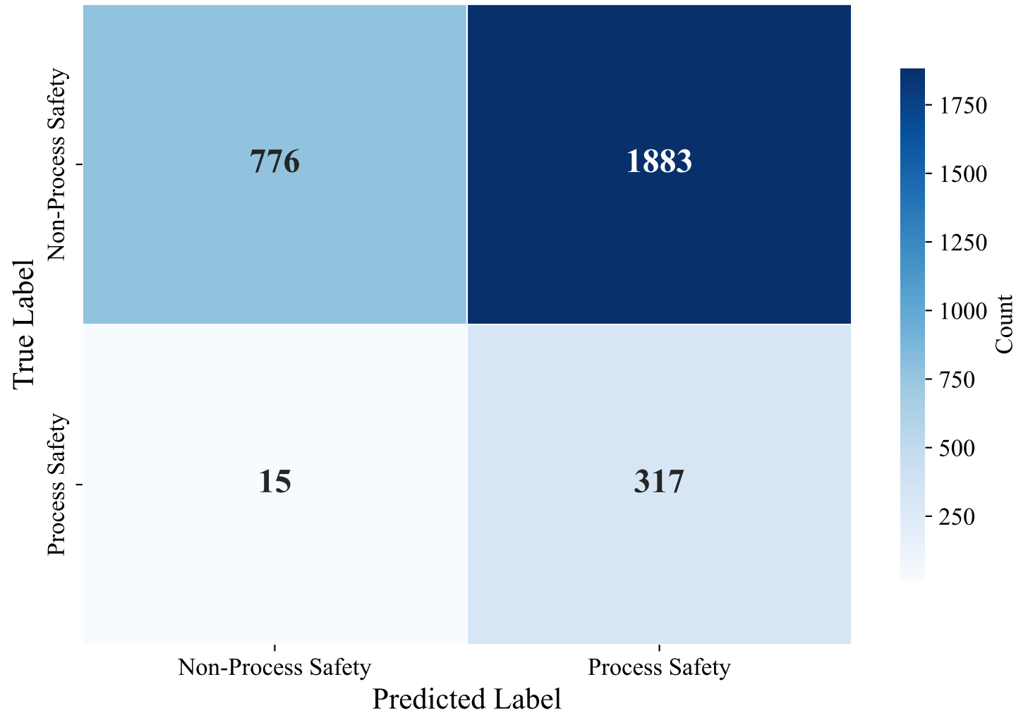
Confusion Matrix — GERMAN_MANUAL (snowflake-arctic-embed-l-v2.0, Random_Forest_Optimized)
