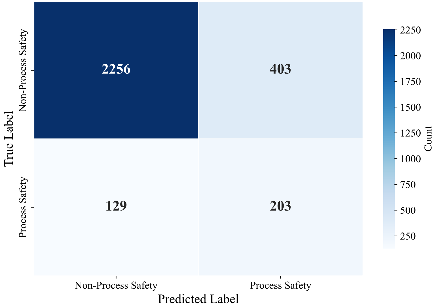
Confusion Matrix — GERMAN_MANUAL (snowflake-arctic-embed-l-v2.0, SVM)
