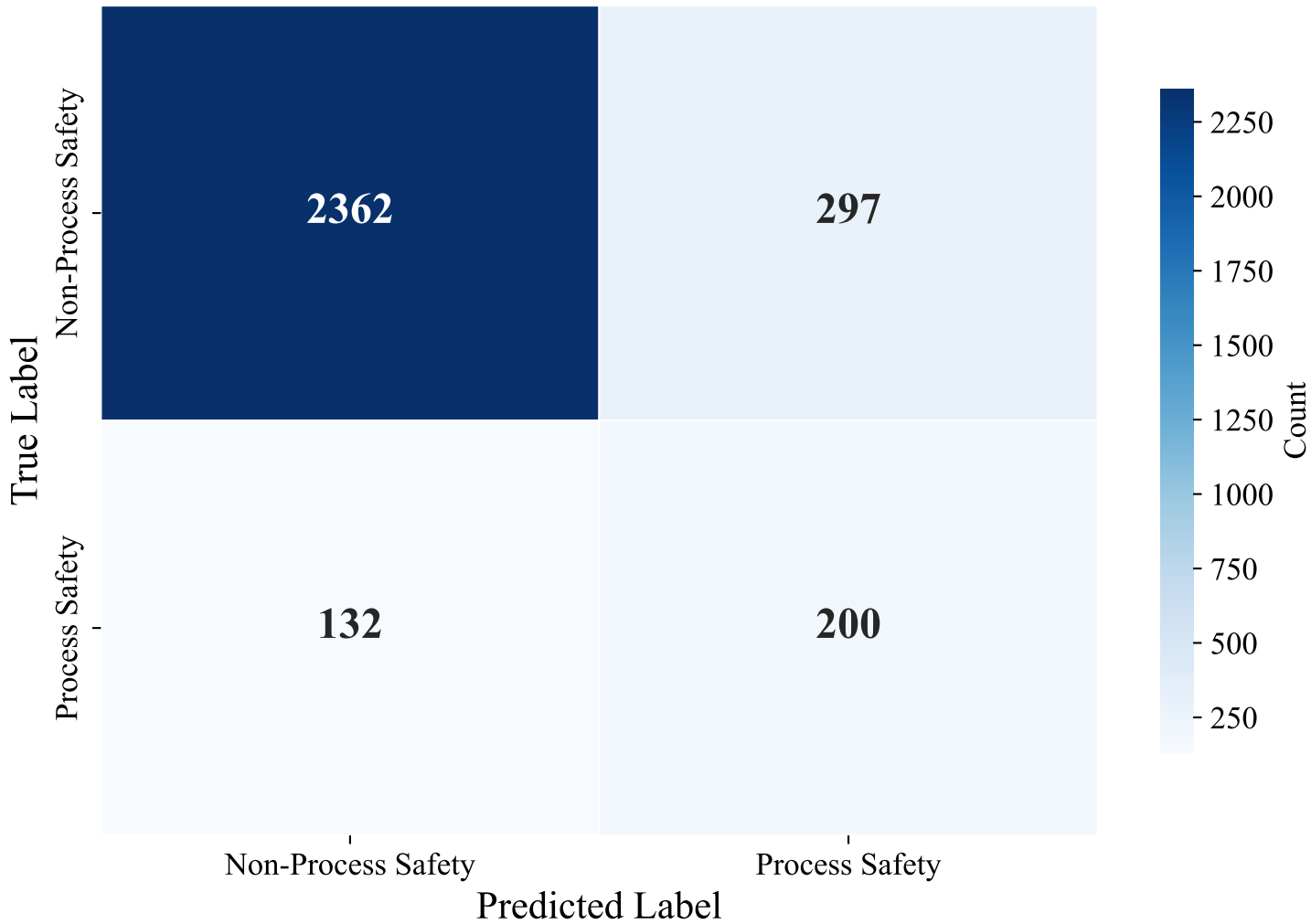
Confusion Matrix — GERMAN_MANUAL (upskyy/bge-m3-korean, LightGBM)
