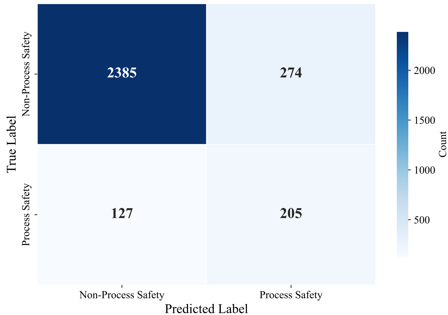
Confusion Matrix — GERMAN_MANUAL (upskyy/bge-m3-korean, XGBoost_Optimized)
