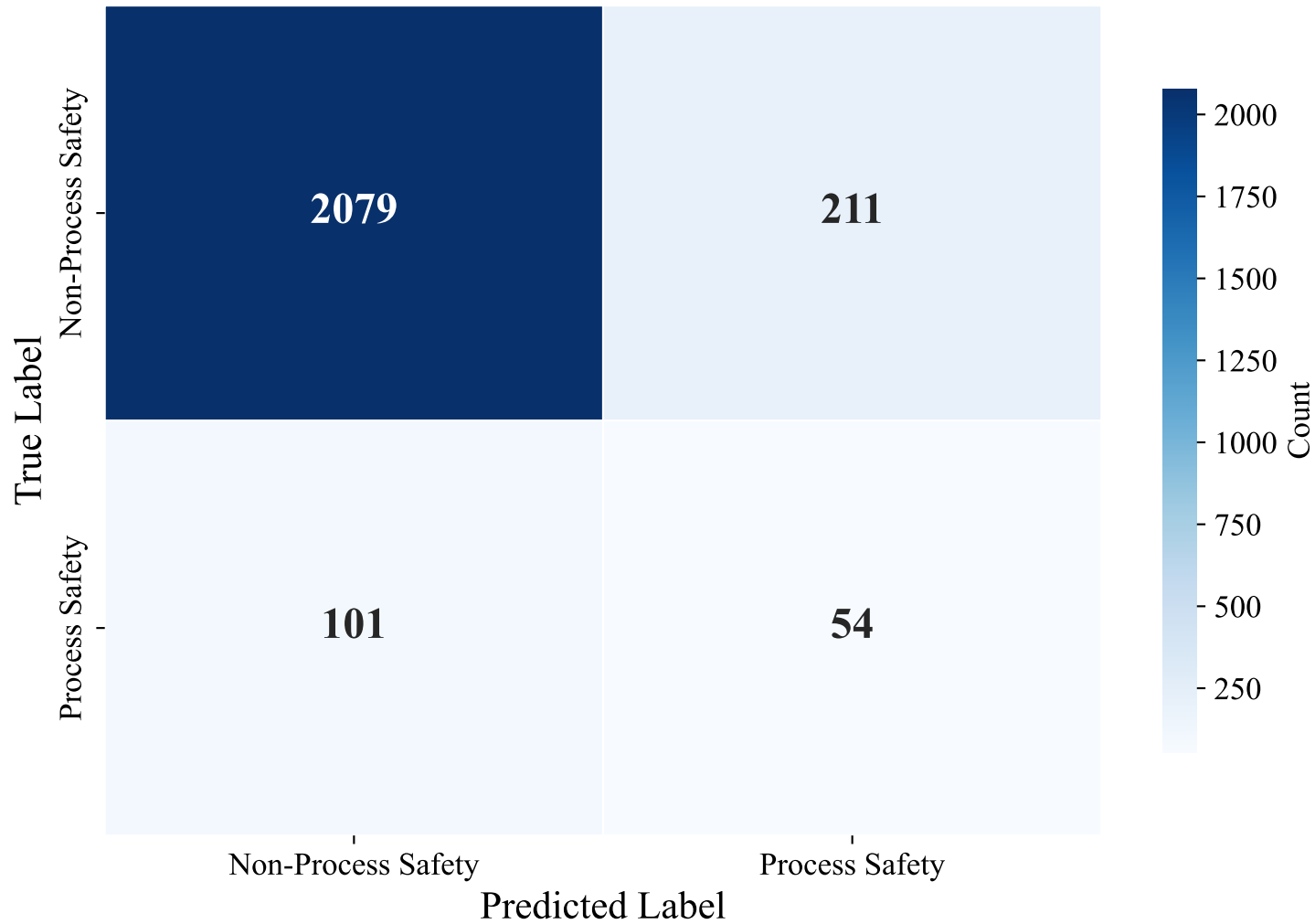
Confusion Matrix — SWEDISH_MANUAL (efederici/e5-base-multilingual-4096, LightGBM_Optimized)
