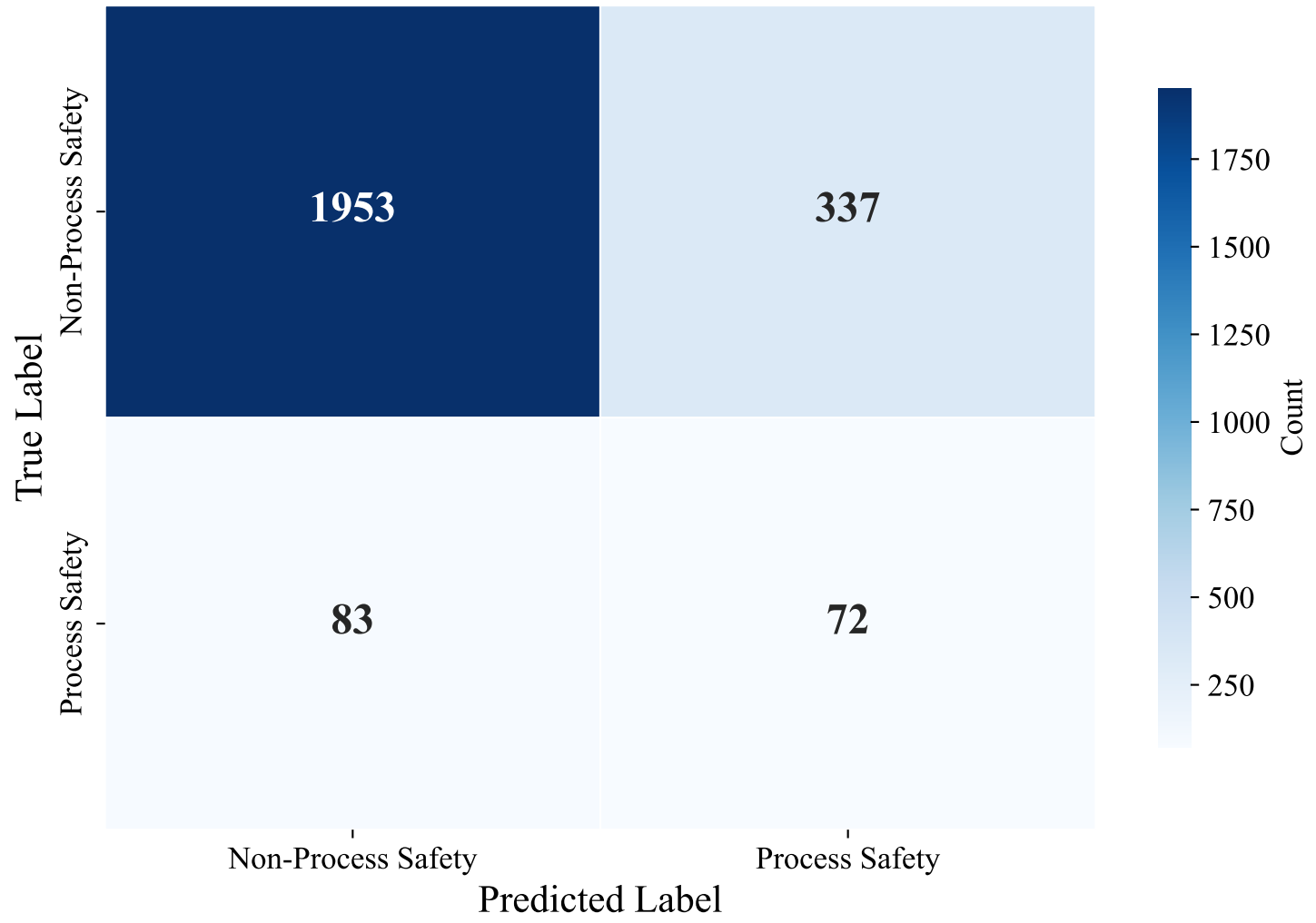
Confusion Matrix — SWEDISH_MANUAL (efederici/e5-base-multilingual-4096, SVM)
