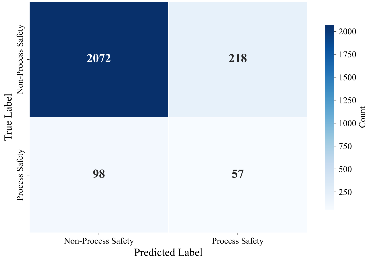
Confusion Matrix — SWEDISH_MANUAL (efederici/e5-base-multilingual-4096, XGBoost)
