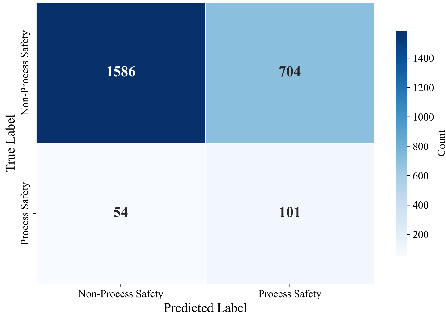
Confusion Matrix — SWEDISH_MANUAL (paraphrase-multilingual-MiniLM-L12-v2, Random_Forest)
