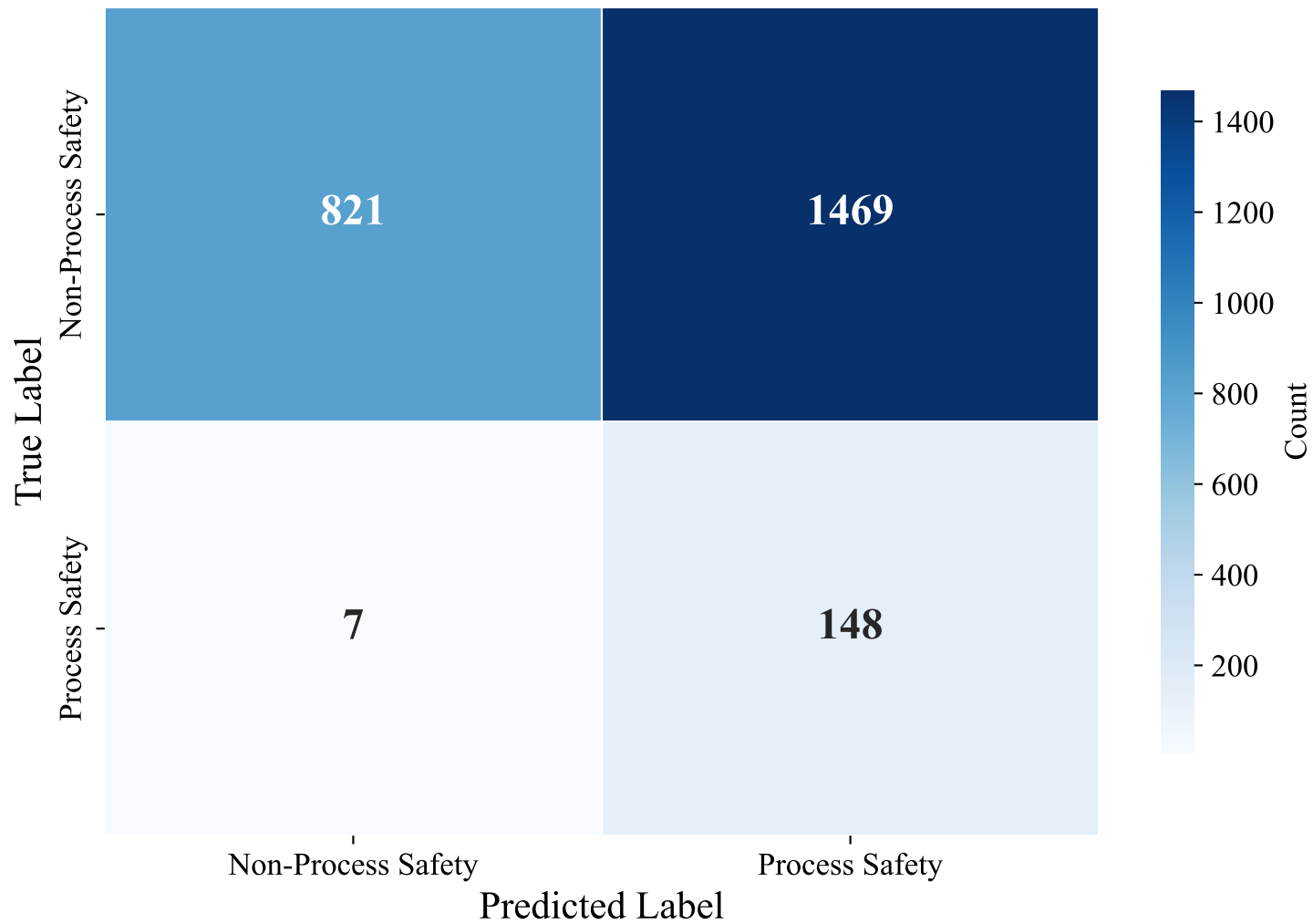
Confusion Matrix — SWEDISH_MANUAL (paraphrase-multilingual-MiniLM-L12-v2, Random_Forest_Optimized)
