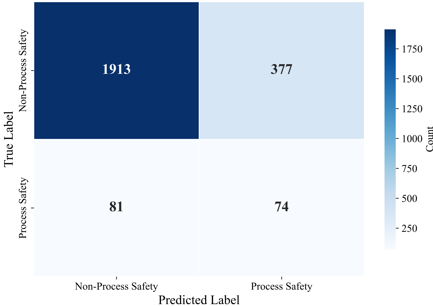
Confusion Matrix — SWEDISH_MANUAL (paraphrase-multilingual-mpnet-base-v2, SVM)
