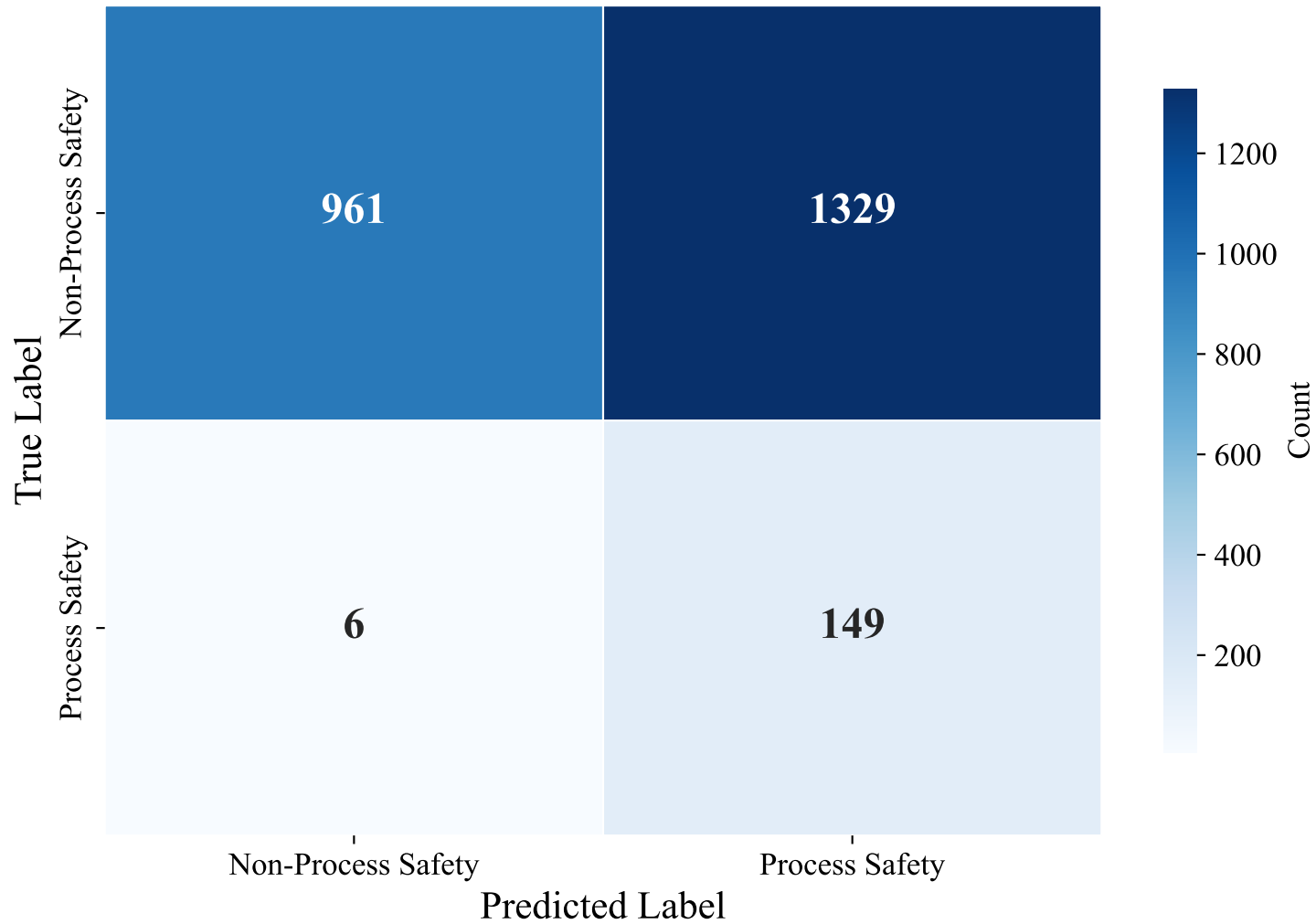
Confusion Matrix — SWEDISH_MANUAL (snowflake-arctic-embed-l-v2.0, Random_Forest_Optimized)
