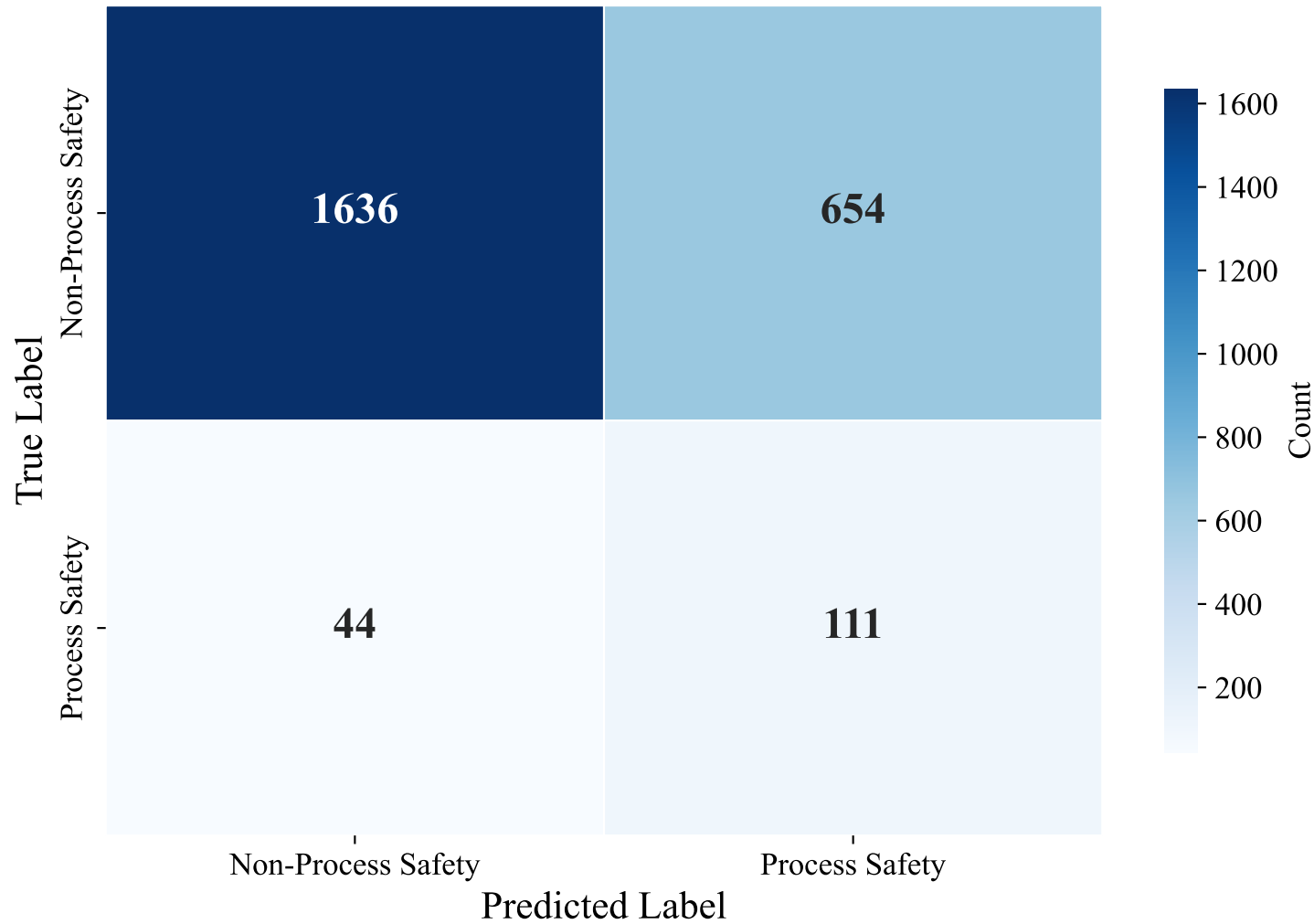
Confusion Matrix — SWEDISH_MANUAL (upskyy/bge-m3-korean, Random_Forest)
