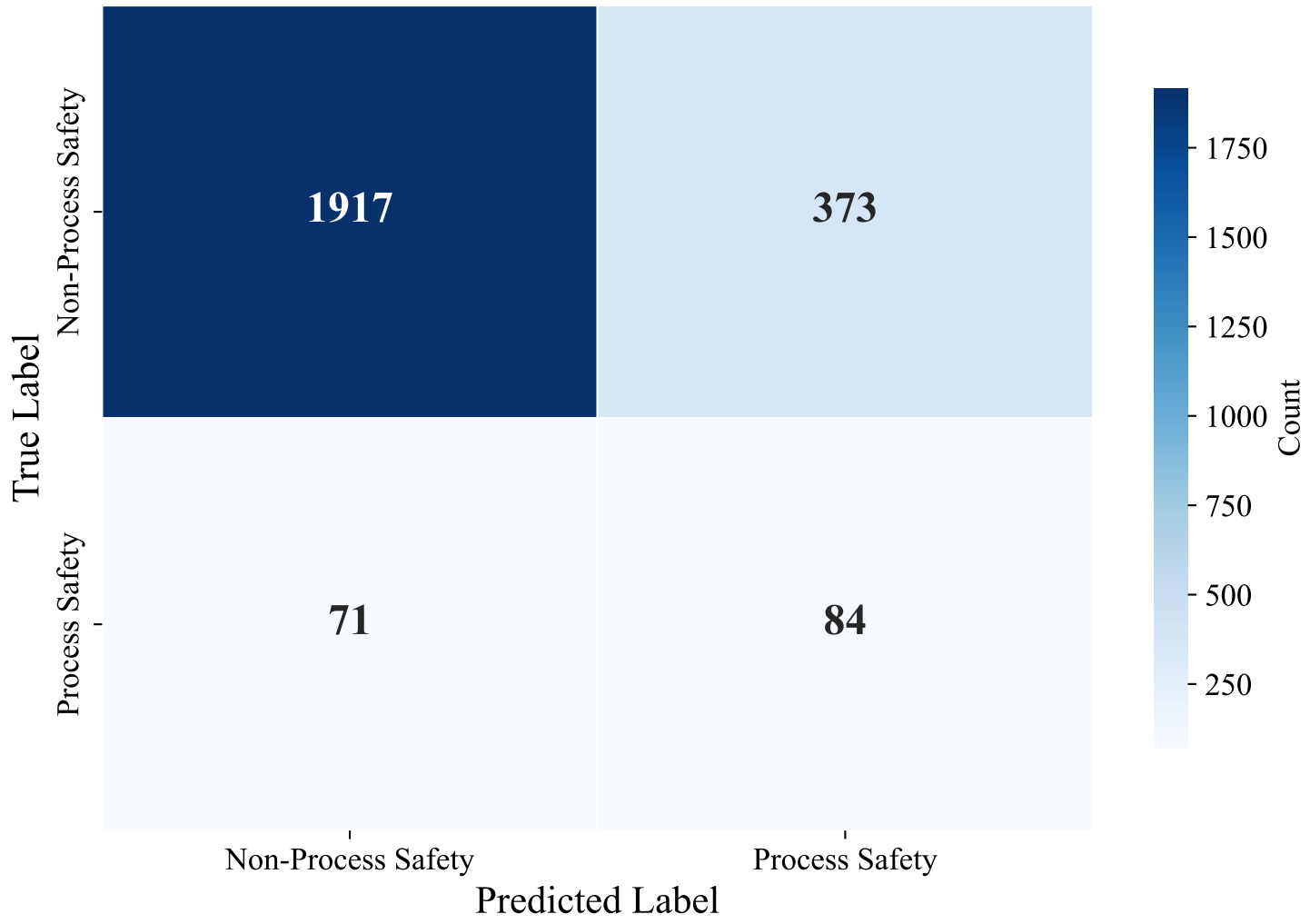
Confusion Matrix — SWEDISH_MANUAL (xlm-roberta-base, SVM)
