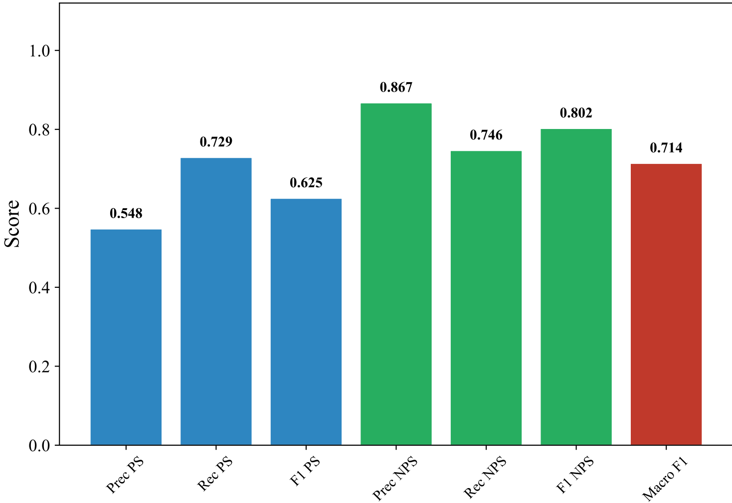
Classification Metrics — DUTCH_MANUAL (efederici/e5-base-multilingual-4096, LightGBM)
