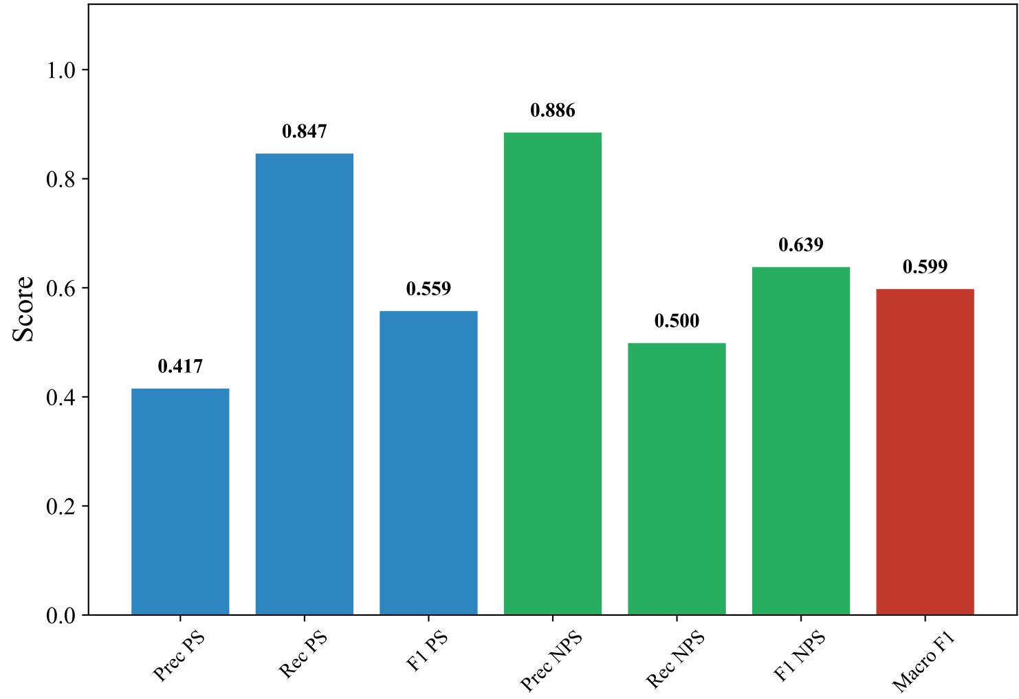
Classification Metrics — DUTCH_MANUAL (efederici/e5-base-multilingual-4096, Random_Forest)
