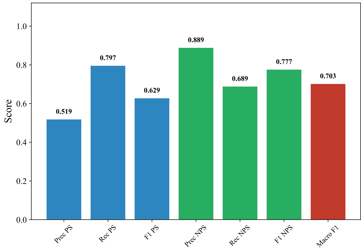
Classification Metrics — DUTCH_MANUAL (efederici/e5-base-multilingual-4096, Voting_Ensemble)
