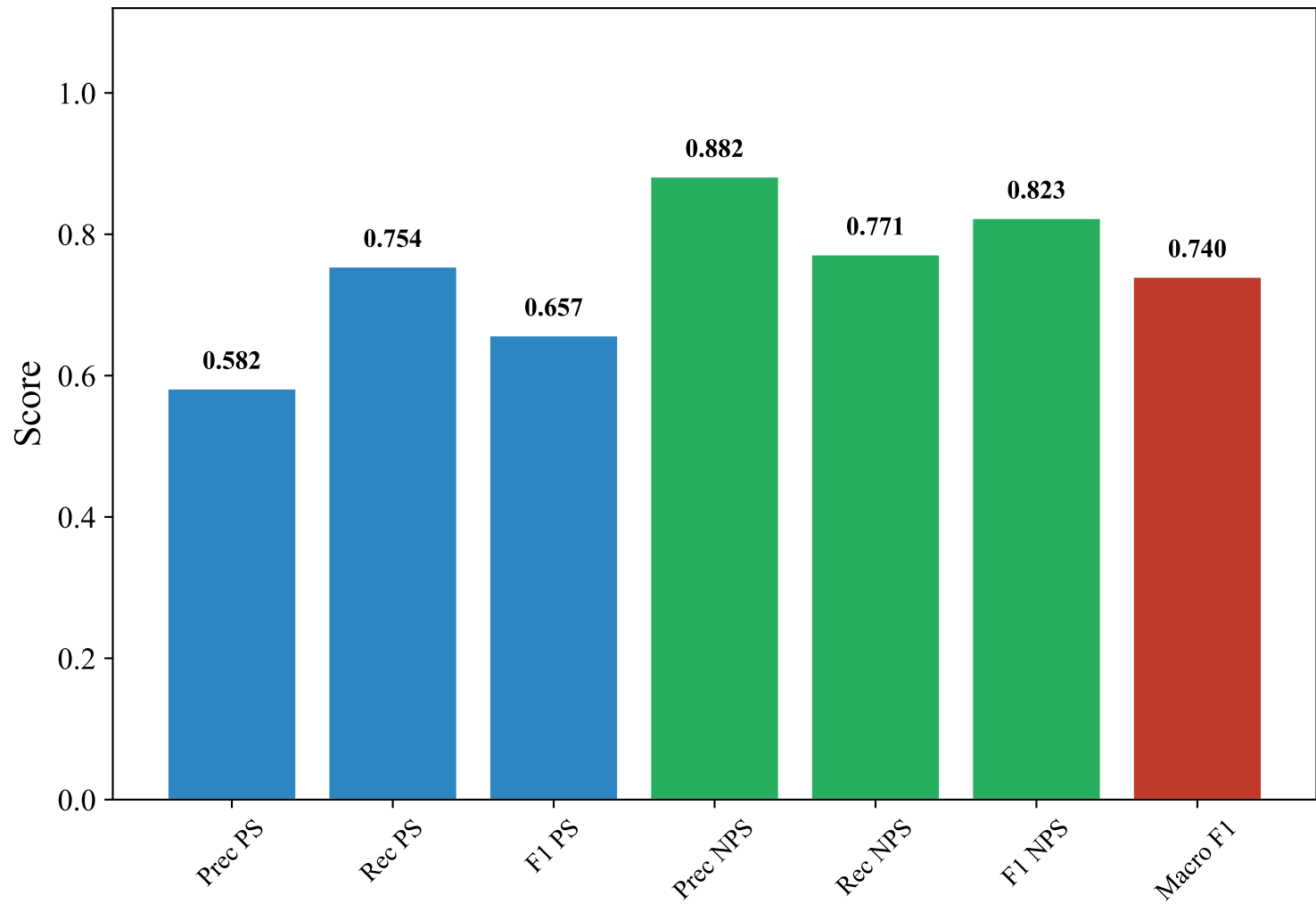
Classification Metrics — DUTCH_MANUAL (intfloat/multilingual-e5-large-instruct, LightGBM_Optimized)
