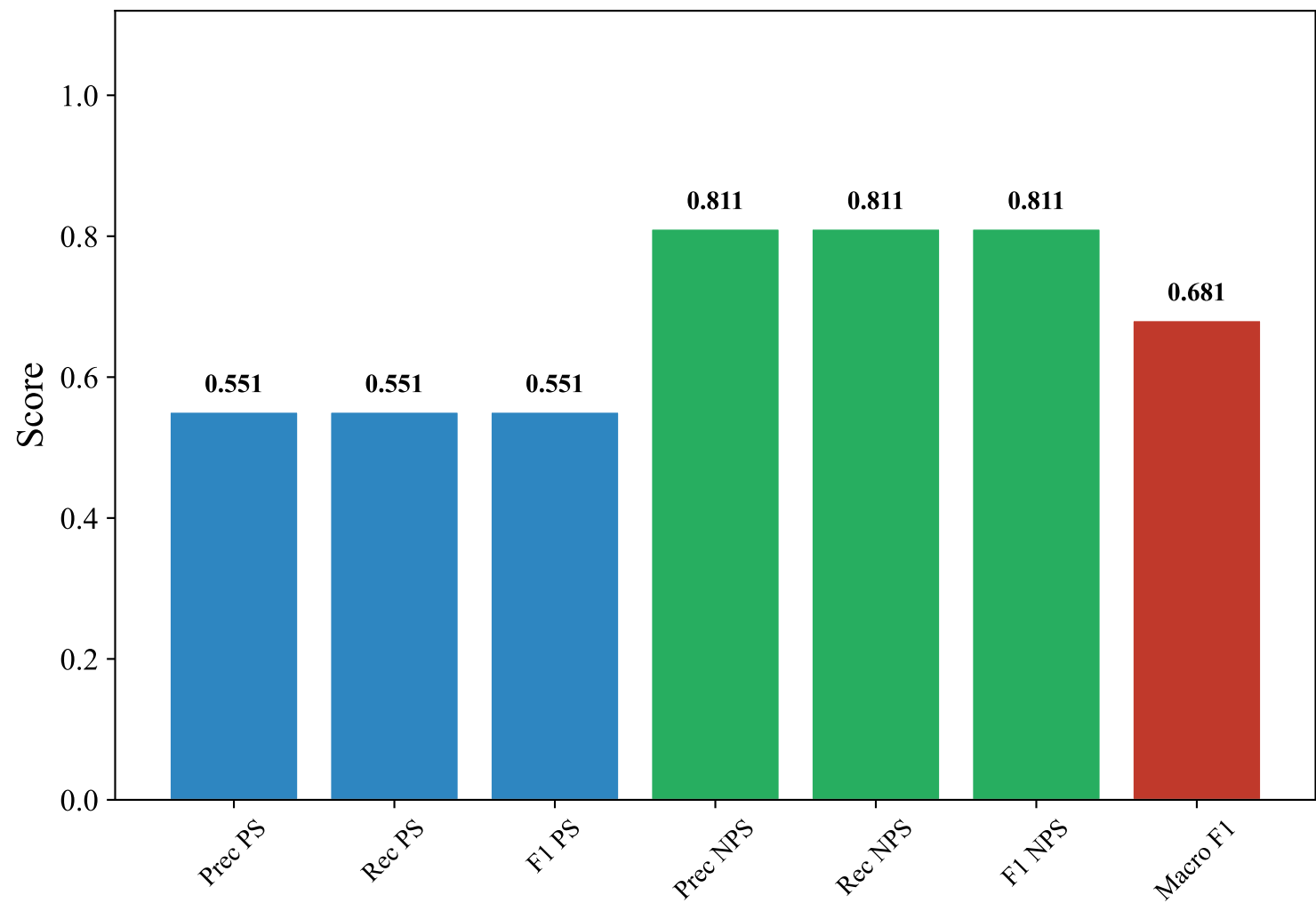
Classification Metrics — DUTCH_MANUAL (intfloat/multilingual-e5-large-instruct, SVM)
