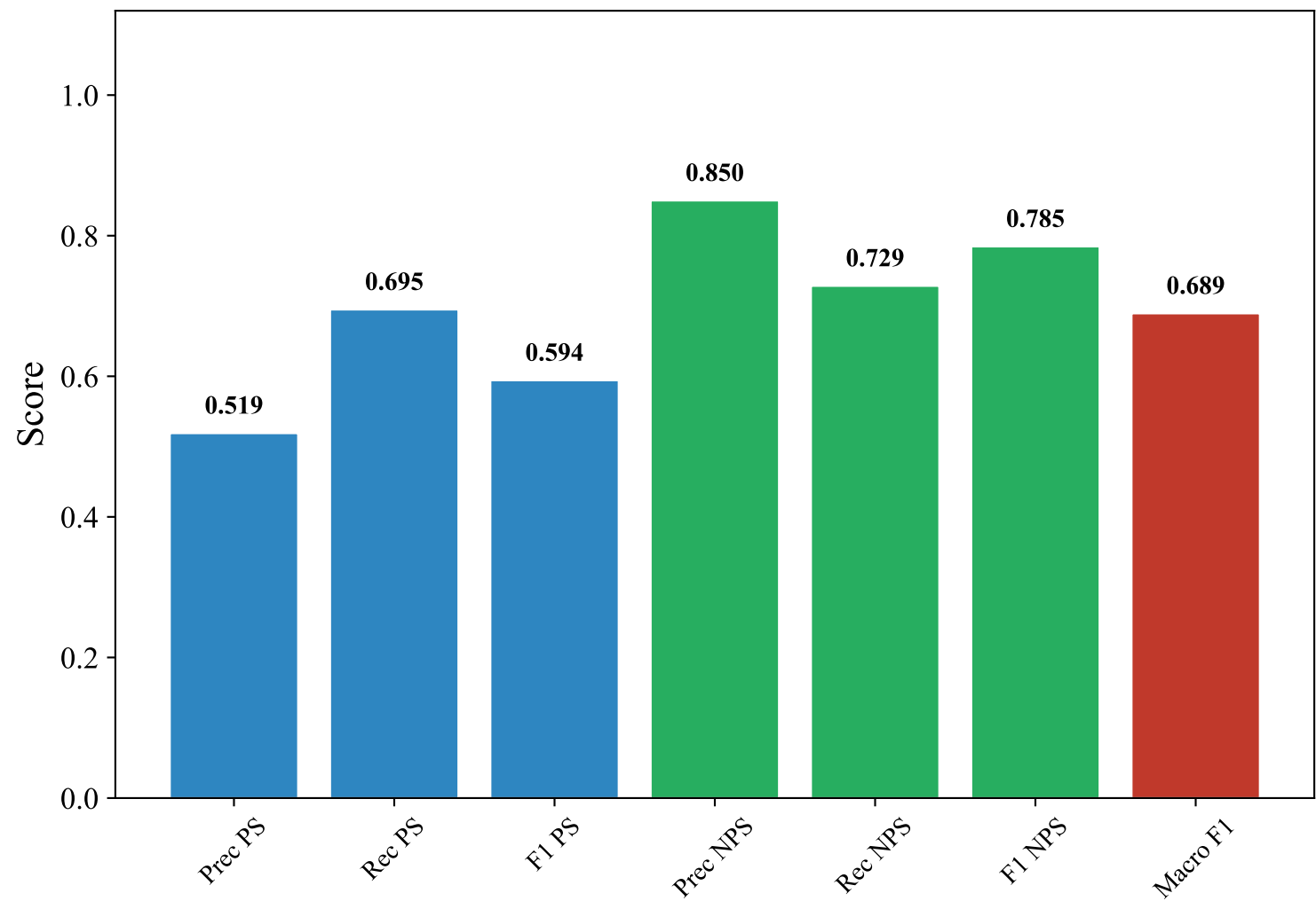
Classification Metrics — DUTCH_MANUAL (paraphrase-multilingual-MiniLM-L12-v2, LightGBM)
