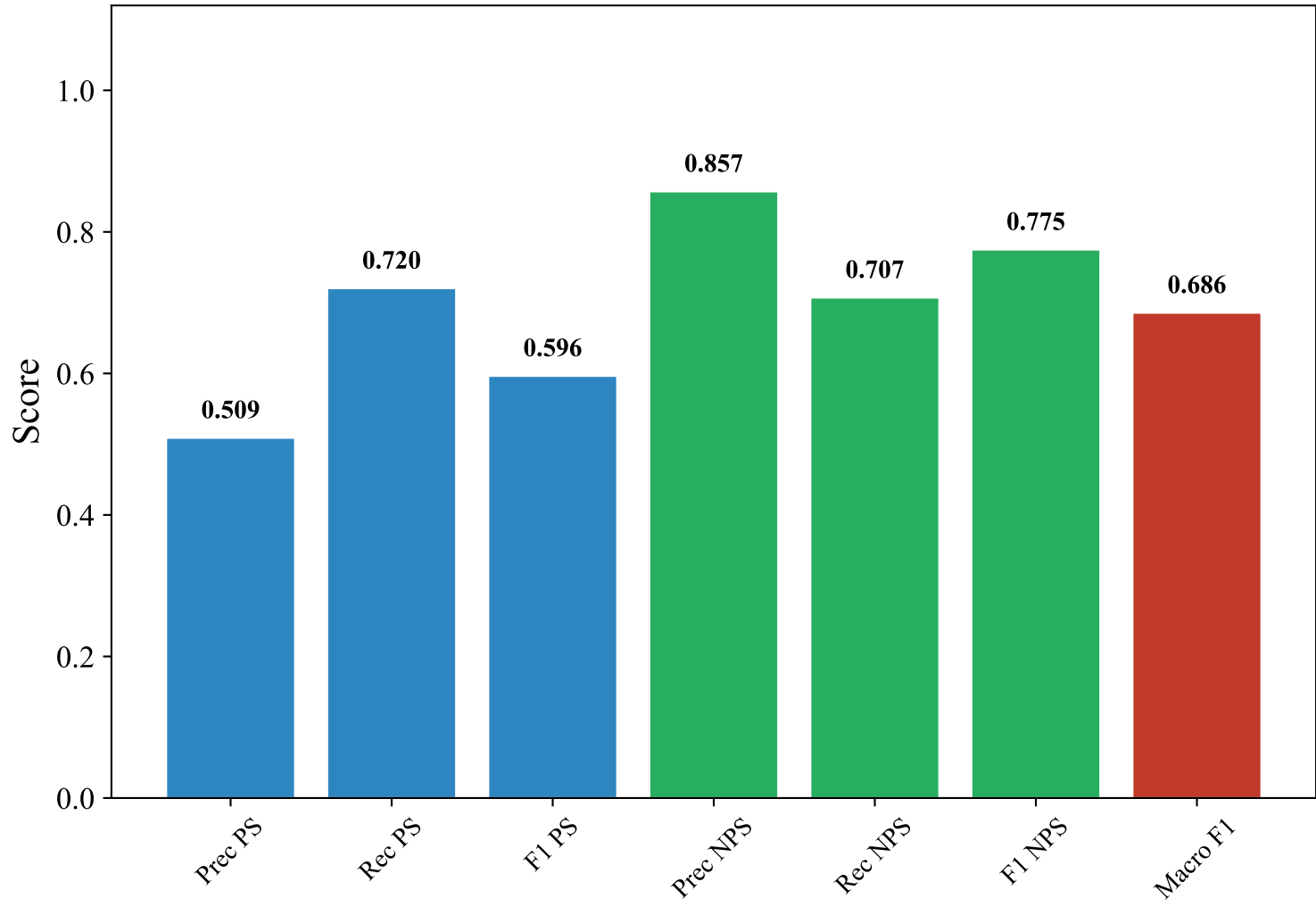
Classification Metrics — DUTCH_MANUAL (paraphrase-multilingual-MiniLM-L12-v2, XGBoost)
