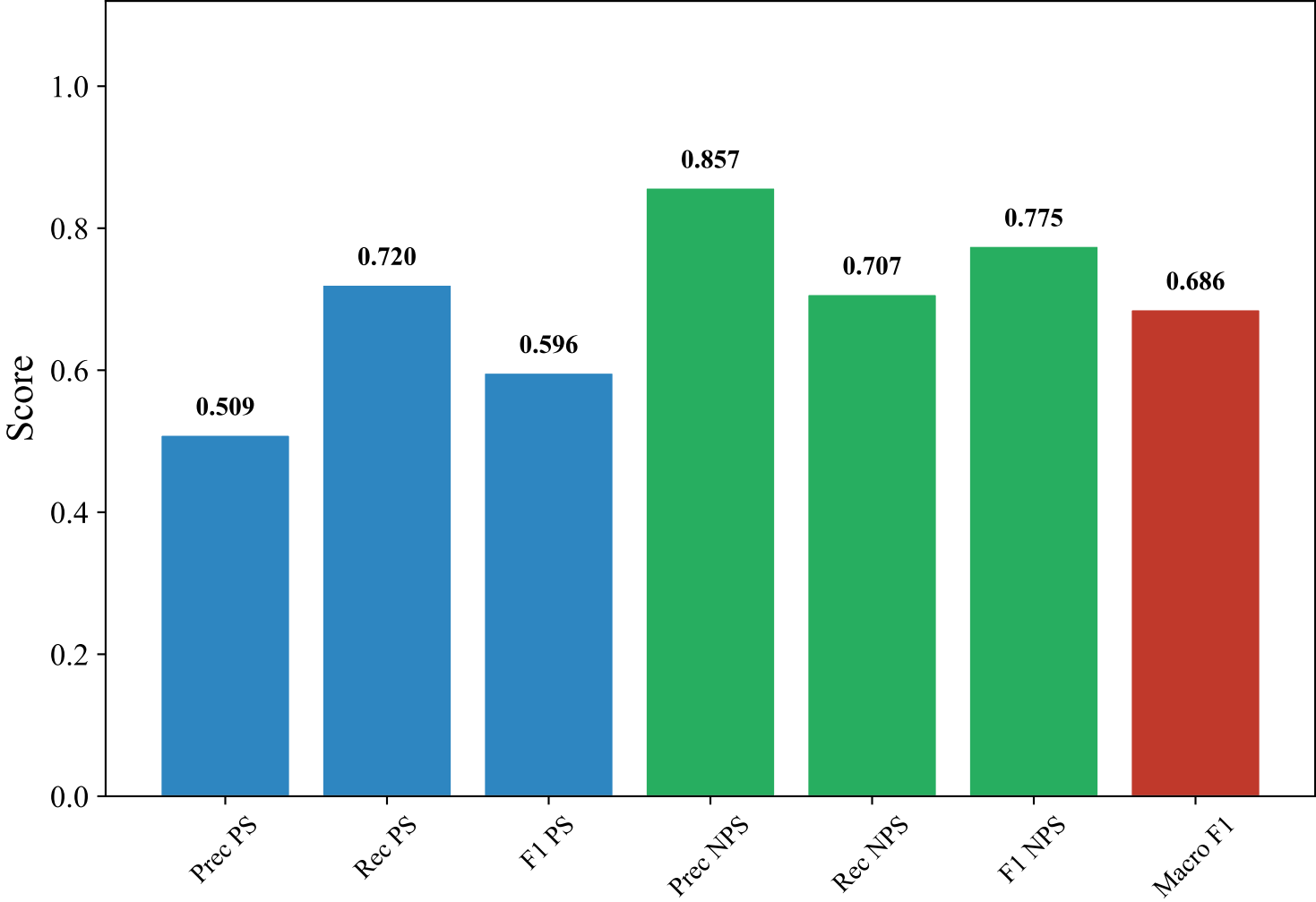
Classification Metrics — DUTCH_MANUAL (paraphrase-multilingual-MiniLM-L12-v2, XGBoost_Optimized)
