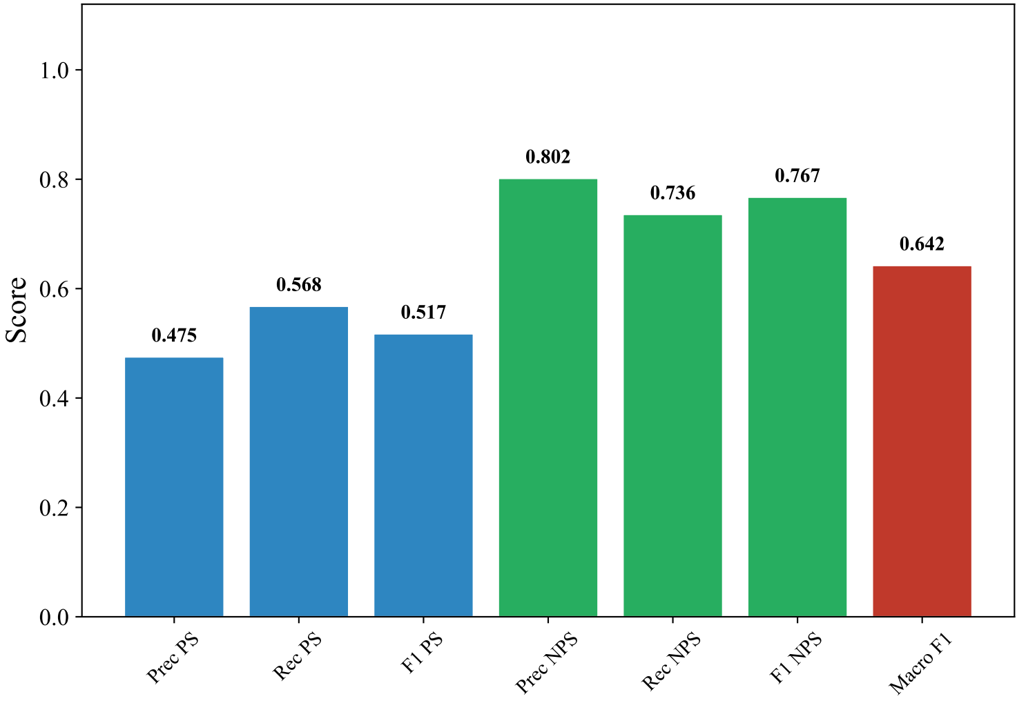
Classification Metrics — DUTCH_MANUAL (snowflake-arctic-embed-l-v2.0, SVM)
