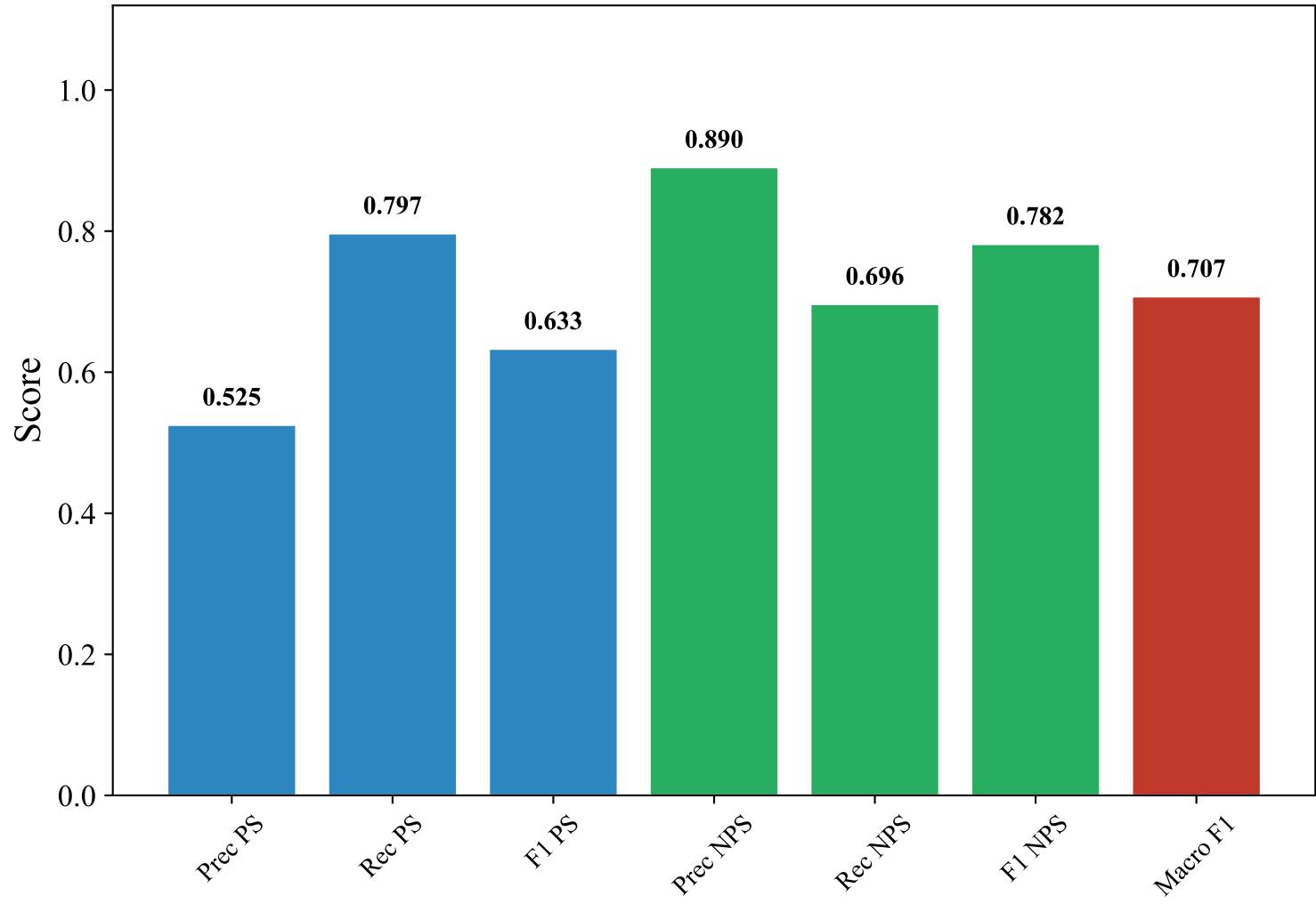
Classification Metrics — DUTCH_MANUAL (snowflake-arctic-embed-l-v2.0, XGBoost)
