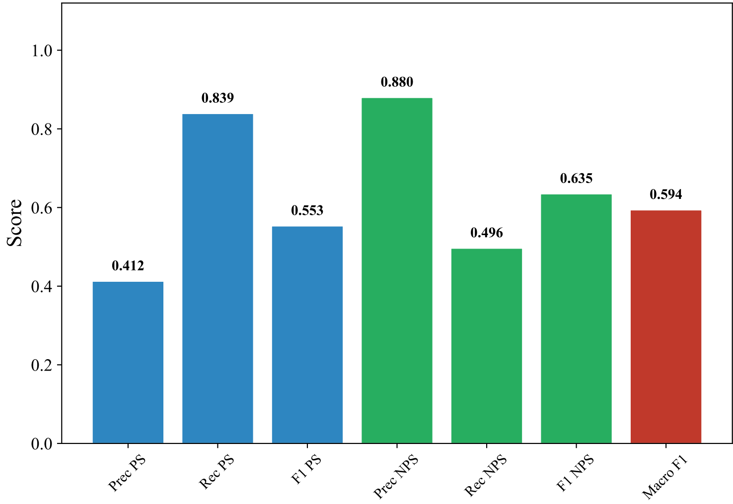
Classification Metrics — DUTCH_MANUAL (upskyy/bge-m3-korean, Random_Forest)
