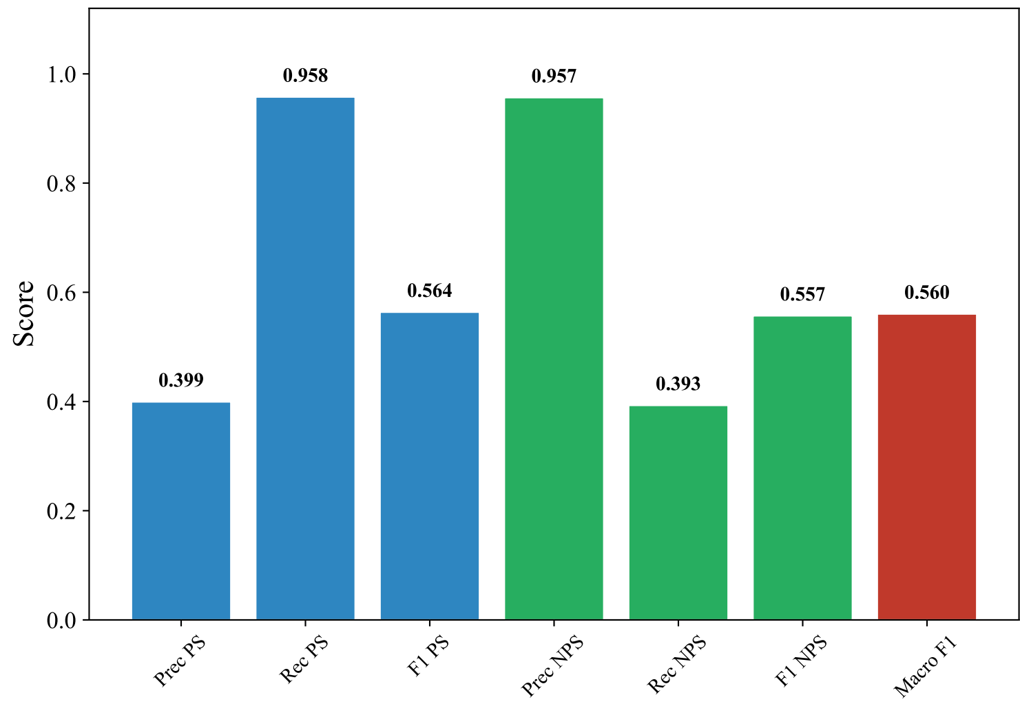
Classification Metrics — DUTCH_MANUAL (xlm-roberta-base, Random_Forest_Optimized)
