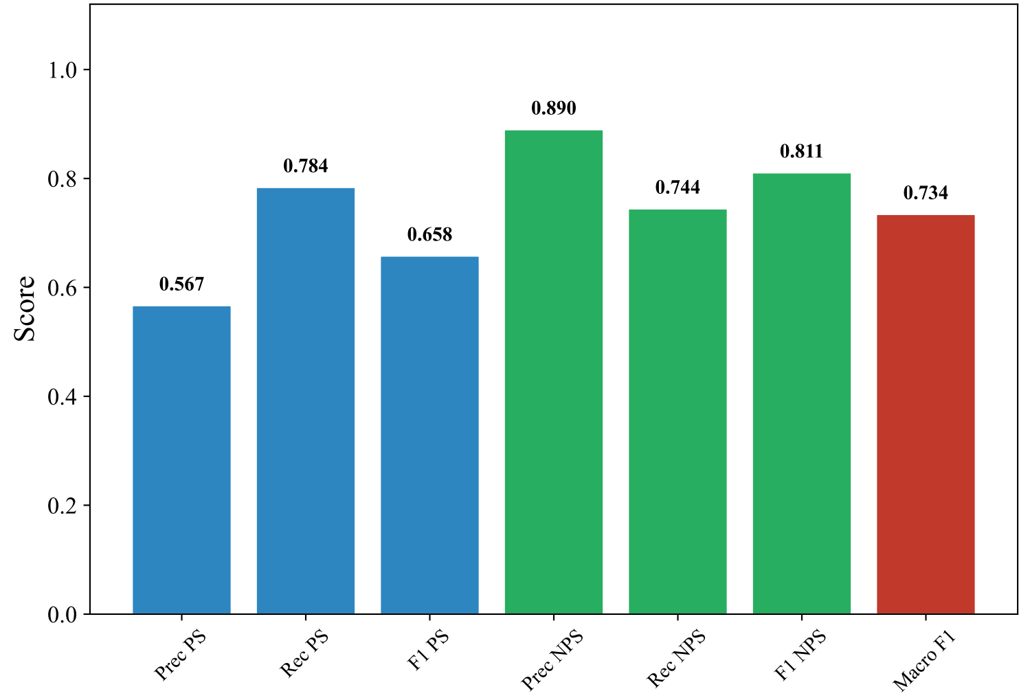
Classification Metrics — ENGLISH_MANUAL (bert-base-multilingual-uncased, XGBoost_Optimized)
