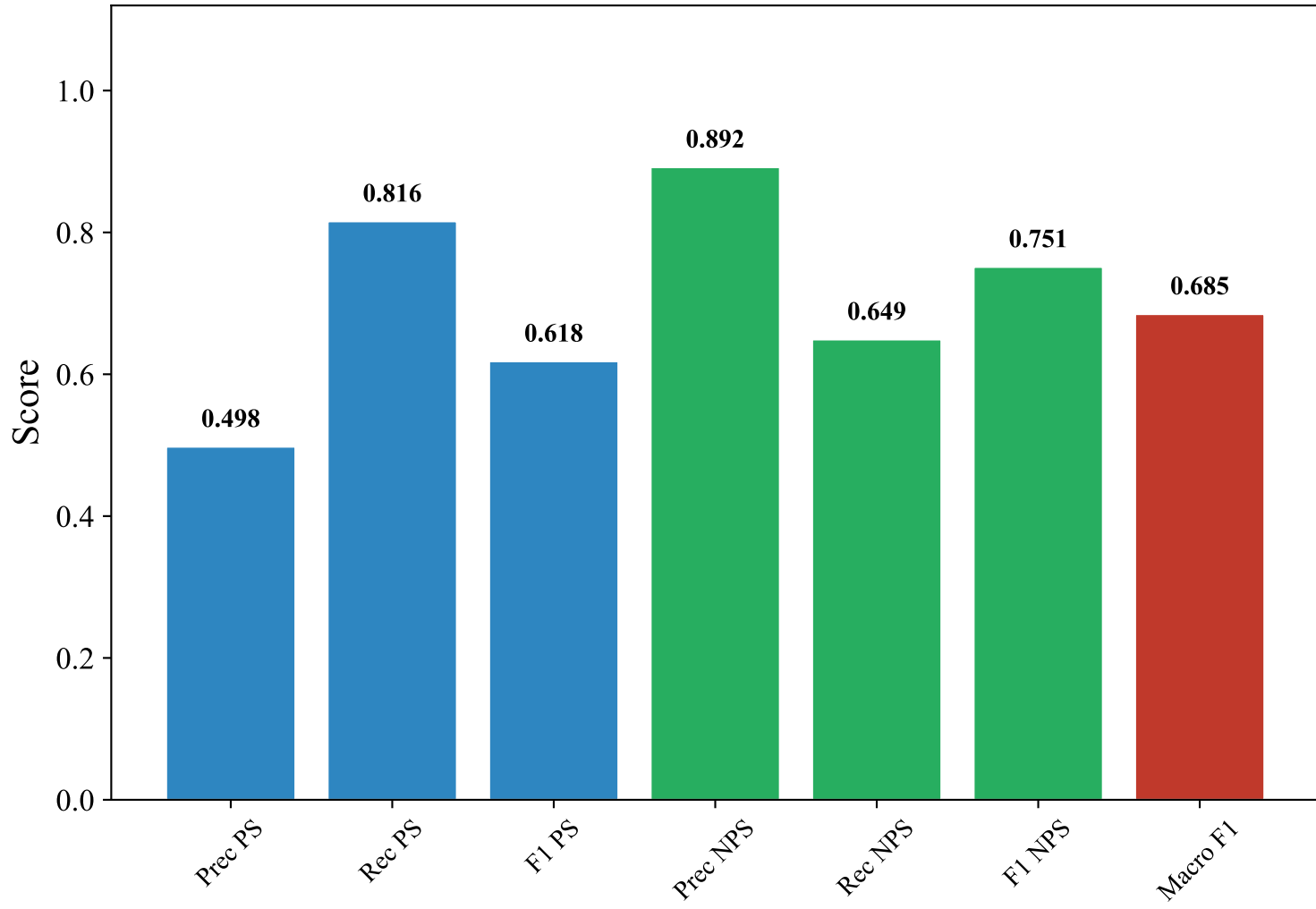
Classification Metrics — ENGLISH_MANUAL (efederici/e5-base-multilingual-4096, Random_Forest)
