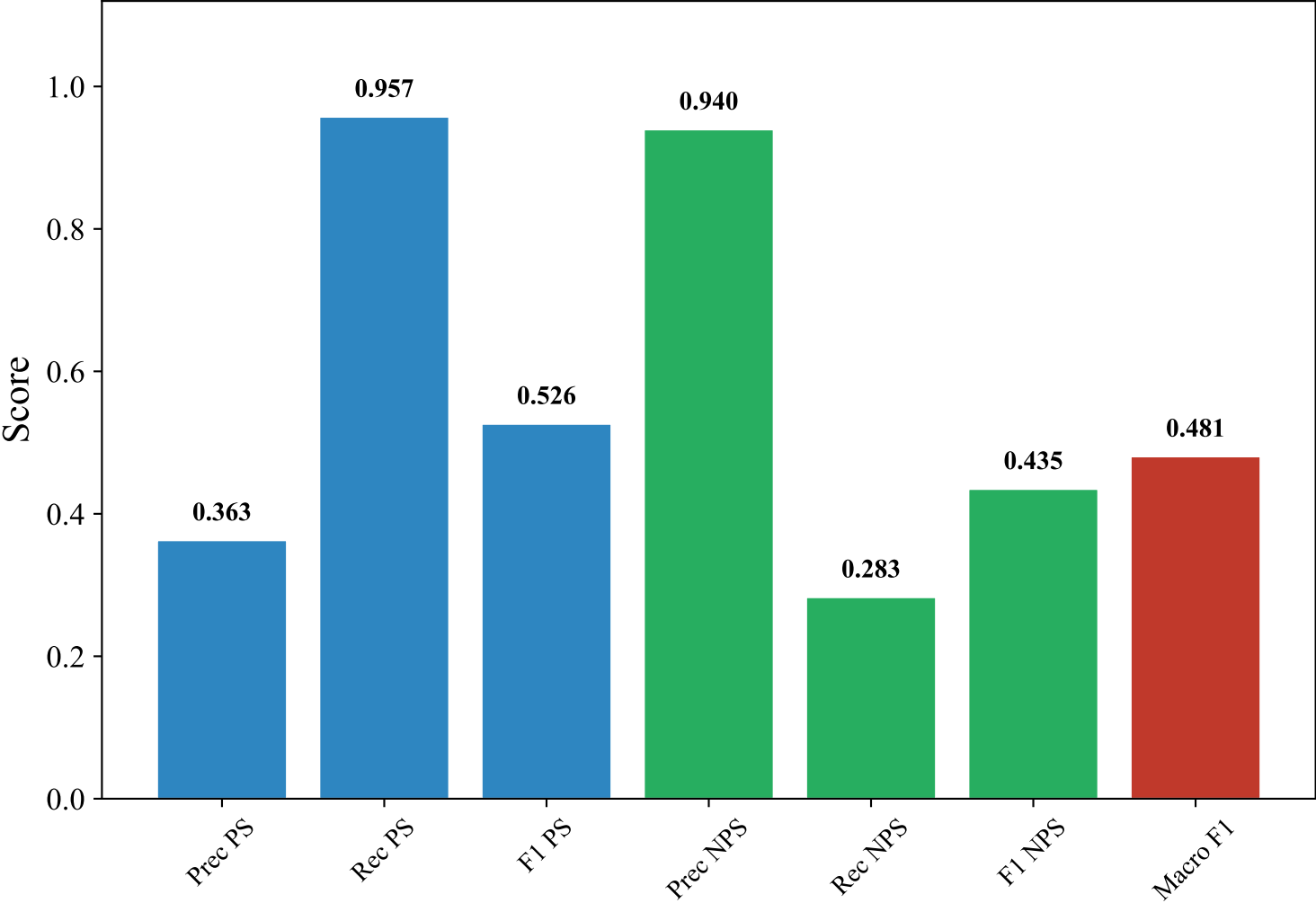
Classification Metrics — ENGLISH_MANUAL (efederici/e5-base-multilingual-4096, Random_Forest_Optimized)
