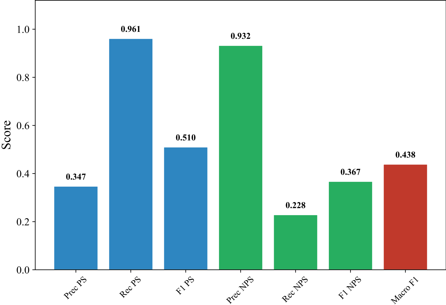
Classification Metrics — ENGLISH_MANUAL (intfloat/multilingual-e5-large-instruct, Random_Forest_Optimized)
