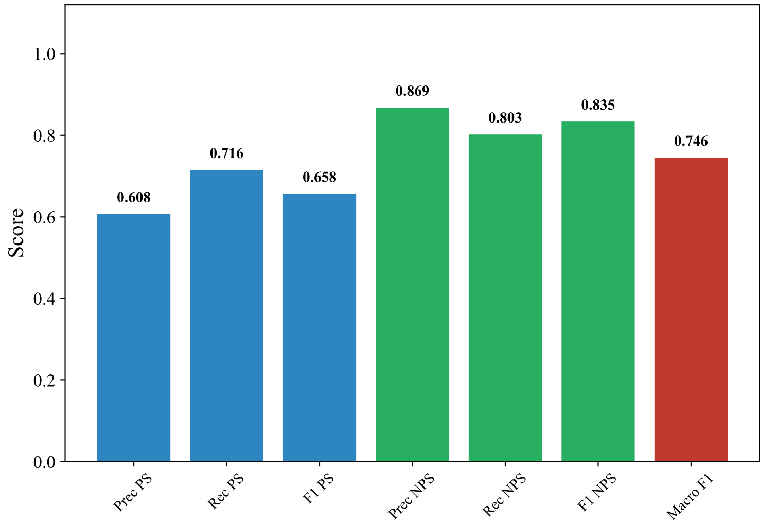
Classification Metrics — ENGLISH_MANUAL (paraphrase-multilingual-MiniLM-L12-v2, SVM)
