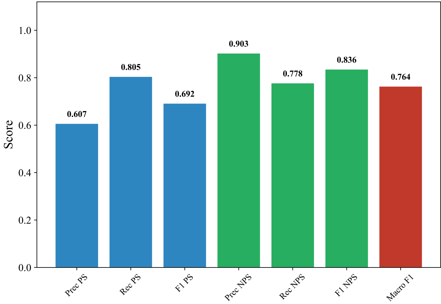
Classification Metrics — ENGLISH_MANUAL (paraphrase-multilingual-mpnet-base-v2, LightGBM)
