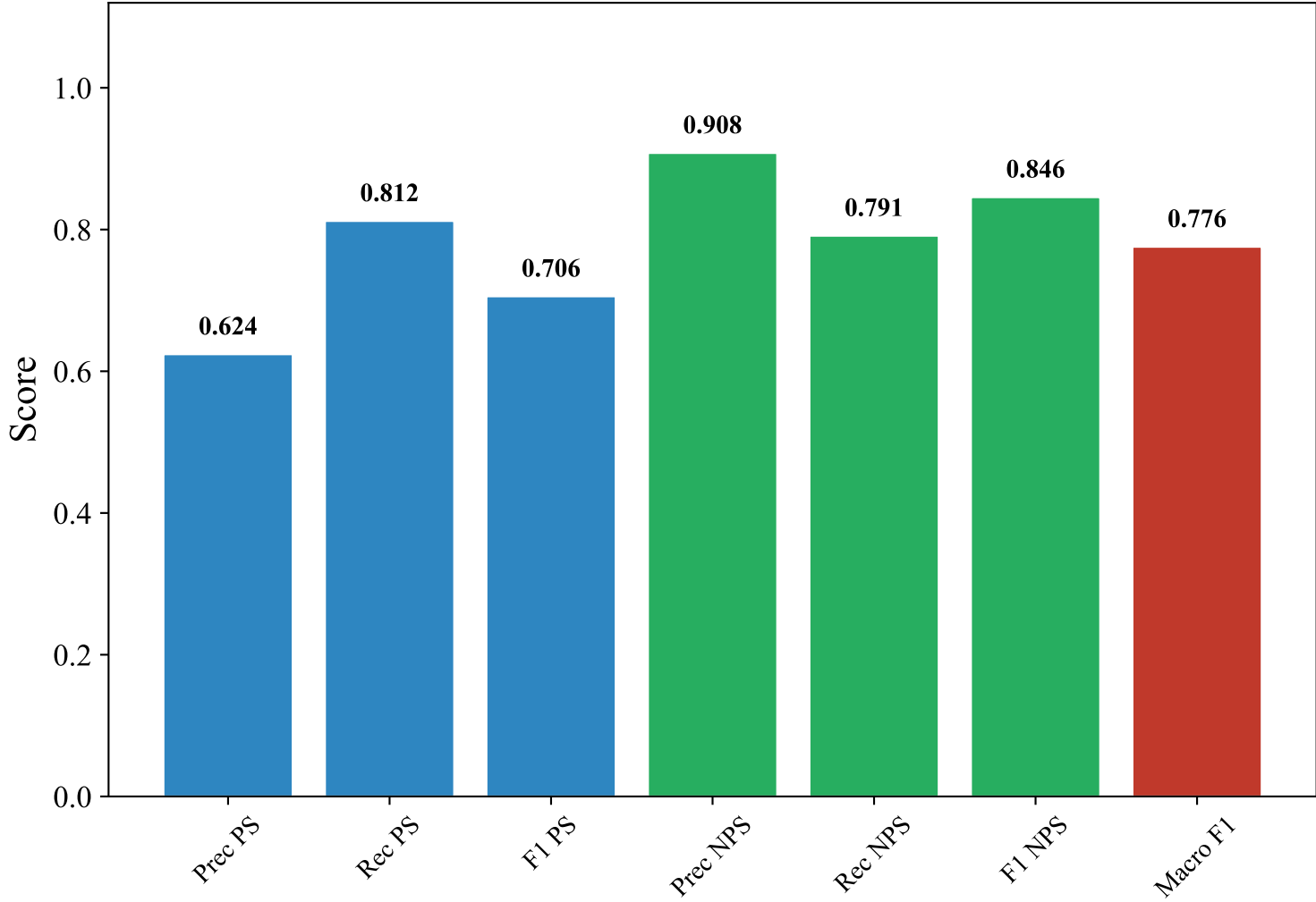
Classification Metrics — ENGLISH_MANUAL (paraphrase-multilingual-mpnet-base-v2, XGBoost_Optimized)
