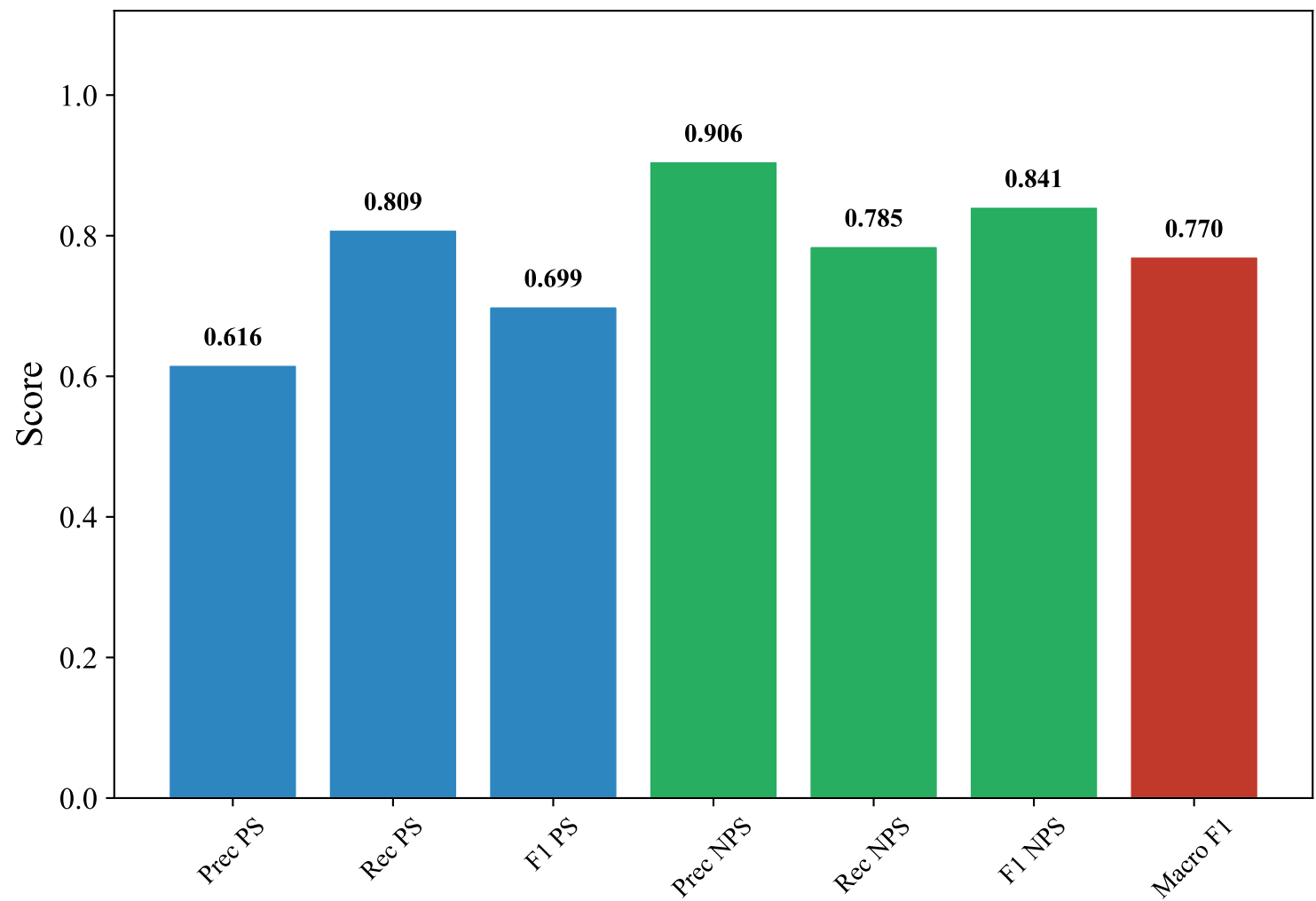
Classification Metrics — ENGLISH_MANUAL (snowflake-arctic-embed-l-v2.0, Voting_Ensemble)
