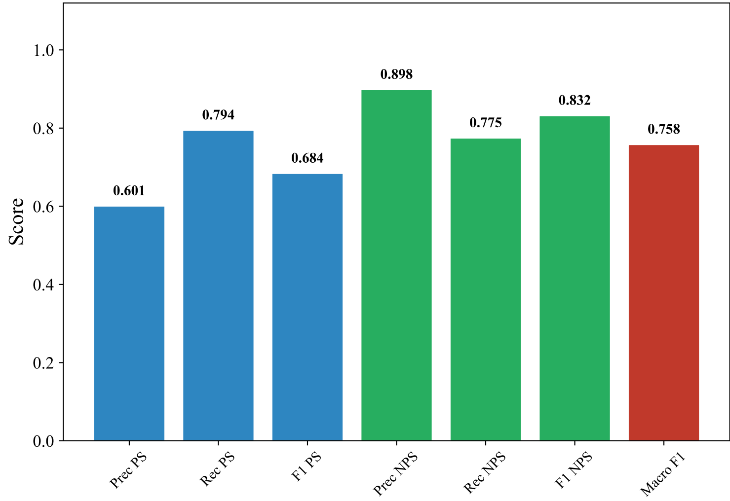
Classification Metrics — ENGLISH_MANUAL (snowflake-arctic-embed-l-v2.0, XGBoost)
