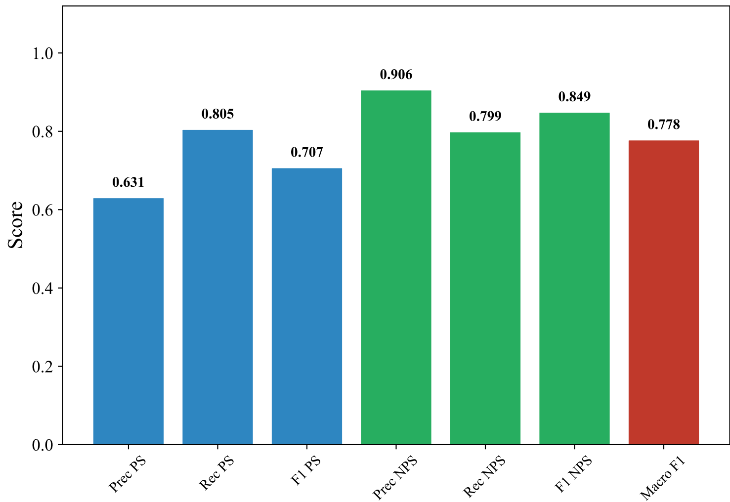
Classification Metrics — ENGLISH_MANUAL (upskyy/bge-m3-korean, LightGBM)
