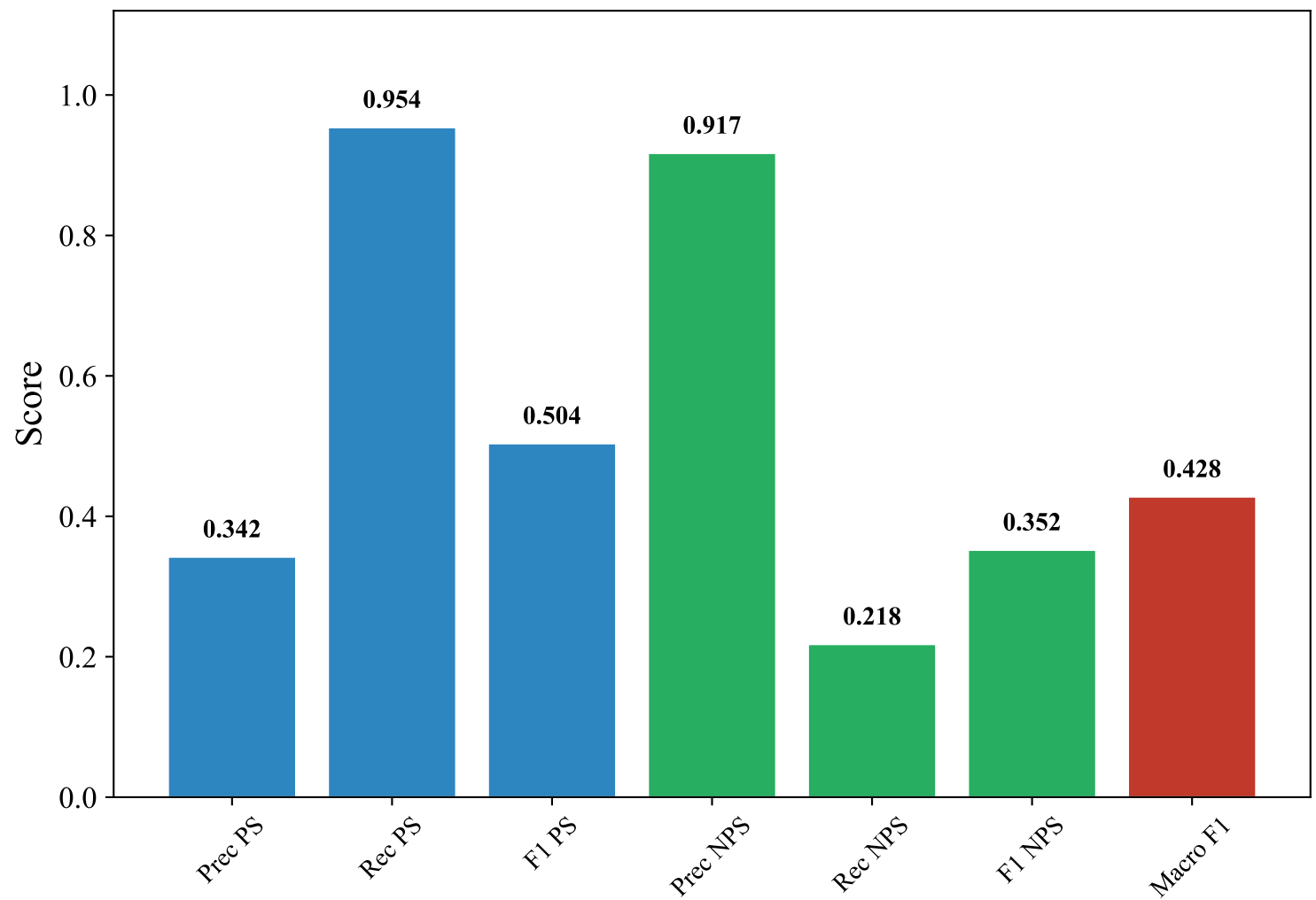
Classification Metrics — ENGLISH_MANUAL (xlm-roberta-base, Random_Forest_Optimized)
